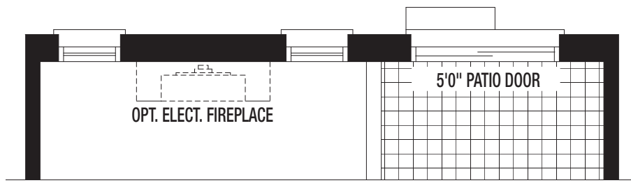
Opt. Partial Plan W/ Elect. Fireplace
